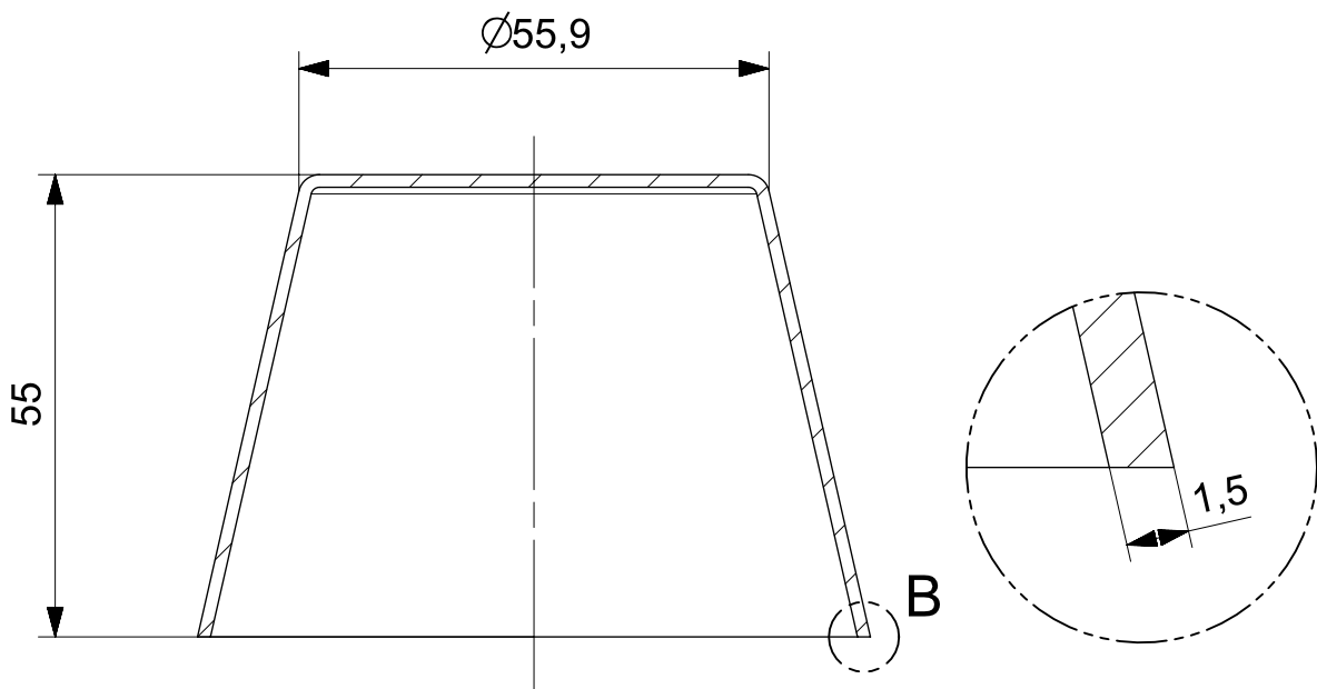
DETAIL B SCALE 5:1
